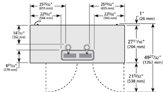
PLAN VIEW
